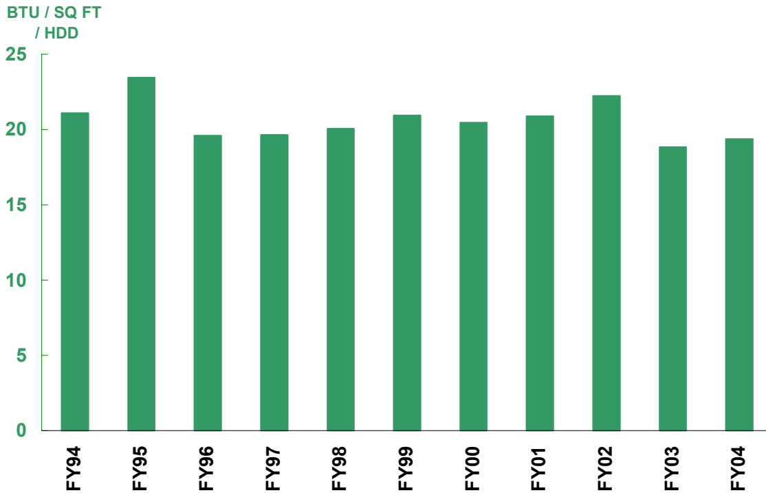
Figure A3 Main campus natural gas consumption normalized for winter weather in HDD and campus growth in square feet
