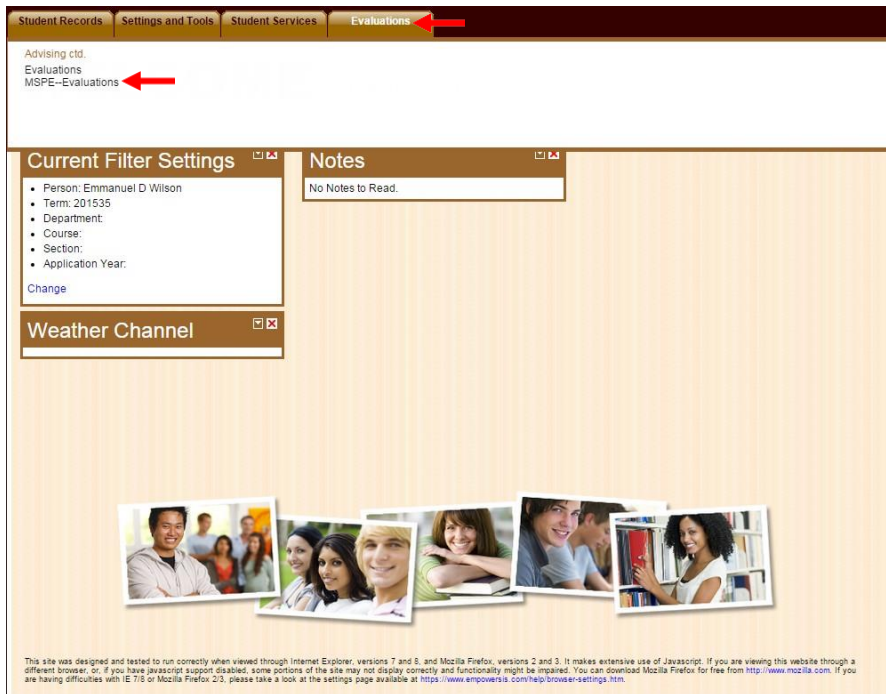
Figure 8: Empower Menu
